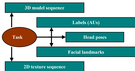
Figure 2: Database organization.
