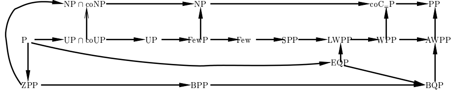
Figure 1. Complexity graph G where a node represents a complexity class and a directed edge (U, V) in G represents the fact that “class U is known to be robustly included in class V .”
