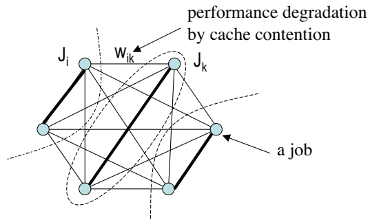
Figure 1: An example of a degradation graph for 6 jobs on 3 dual-cores. Each partition contains a job group sharing the same cache. Bold edges compose a perfect matching.
