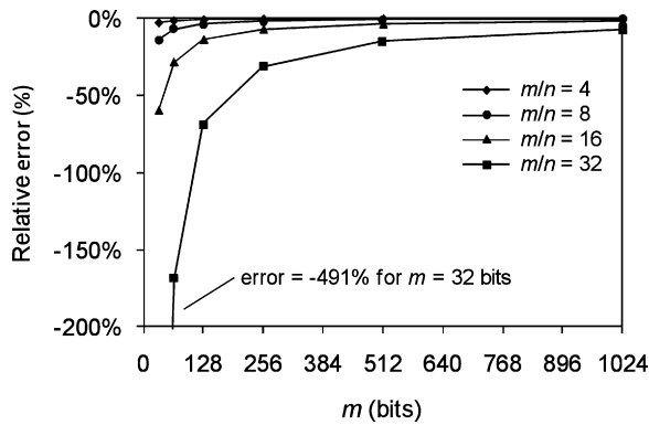
Fig. 2. Relative error of classic versus new formula.
