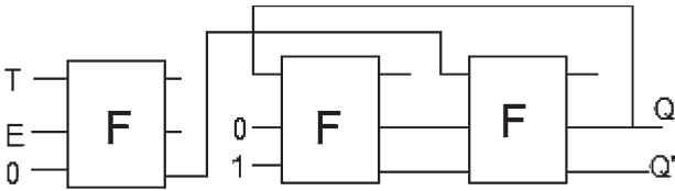
Fig. 6. Concurrently testable T latch design.
