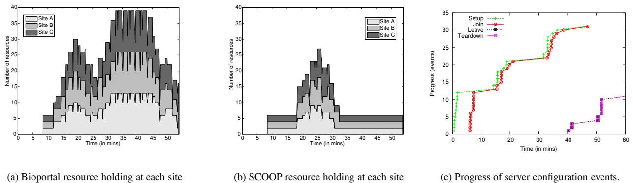
Figure 5: Site resources are allocated to competing GROC according to their configured priorities. (a) shows the decrease in resources available to Bioportal as more machines are reserved to SCOOP, as shown in (b). Bioportal reacquires the machines as SCOOP releases them. (c) shows the progress of resource configuration events on sites and GROC.
