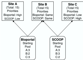
Figure 3: The testbed has three cluster sites with a maximum capacity of 15 virtual machines each. There are two hosted grids (the Biportal and SCOOP applications). Each site assigns a priority for local resources to each grid, according to its local policies.
