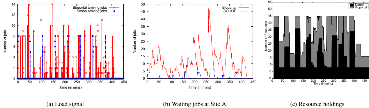
Figure 6: Adaptive provisioning under varying load. The load signal (a) gives job arrivals. (b) shows the waiting jobs queue at Site A, while (c) shows a stacked plot of the resource holdings of each grid across the three sites.
